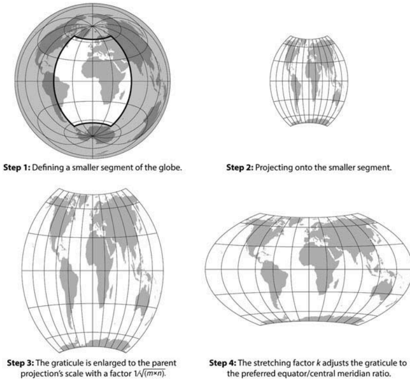
Figure 3. Wagner's steps in deriving the Wagner VII projection from the Lambert azimuthal equal-area projection using his transformation method (after Wagner 1941).
