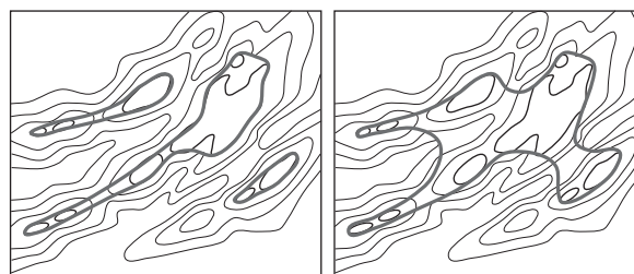
Fig. 2. Medium (left) and strong (right) aggregation of small mountain peaks (Horn, 1945).
