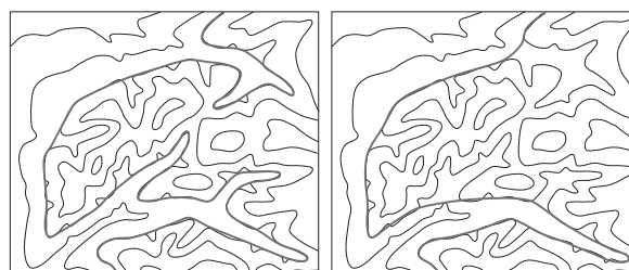
Fig. 3. Medium (left) and strong (right) generalisation of valleys (Horn, 1945).
